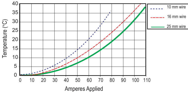
EBC80 Series Temperature Rise at Constant Current
