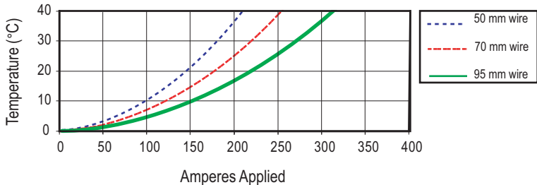
EBC320 Series Temperature Rise at Constant Current
