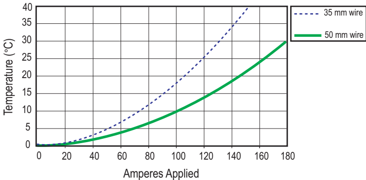
EBC160 Series Temperature Rise at Constant Current
